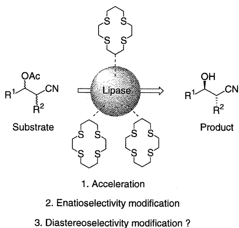
Fig. 1. Thiocrown ether modification of lipase-catalyzed reaction.
